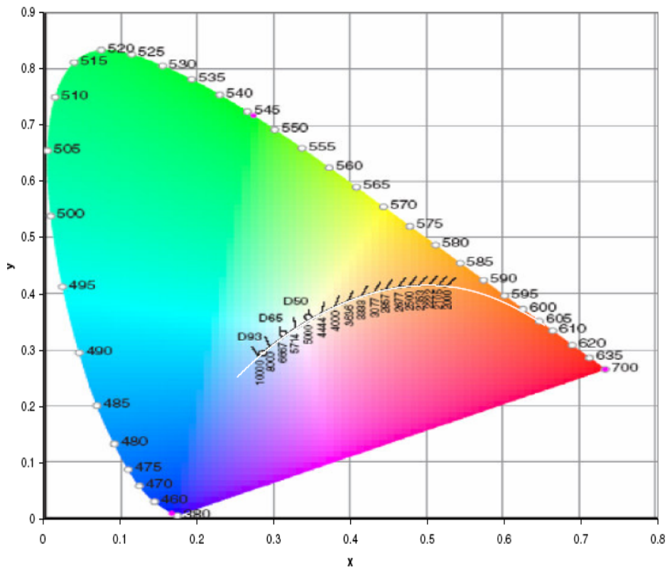
Figure 9. CIE 1931 Diagram
