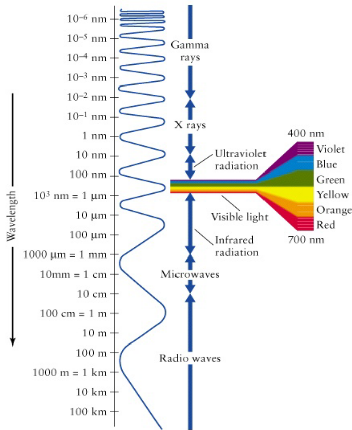
Figure 1. Electromagnetic radiation
