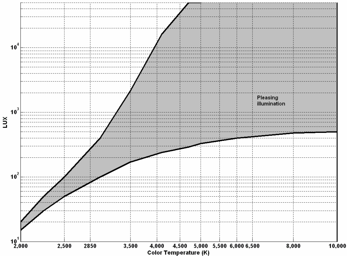
Figure 7. Kruithof Curve
