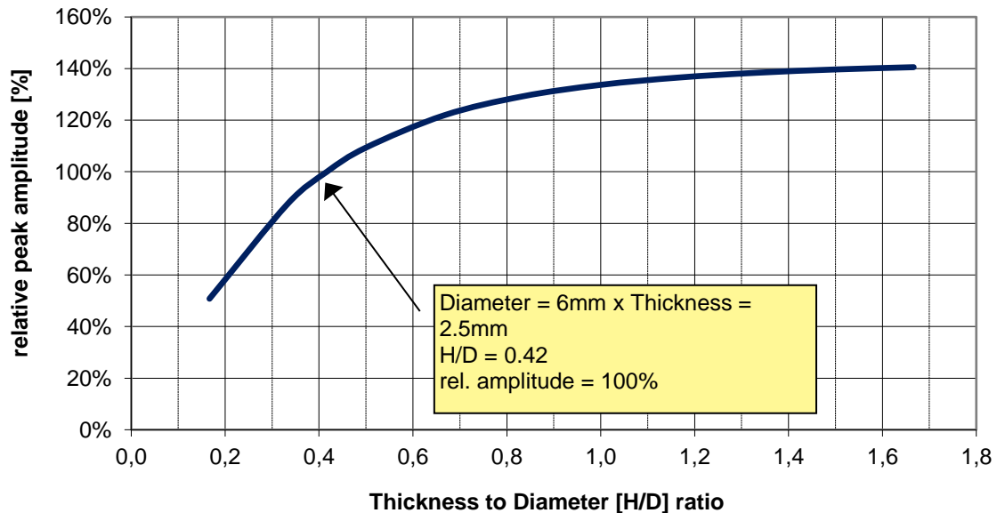
Figure 15 Thickness/Diameter Ratio
