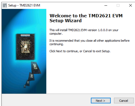
Figure 2: Welcome Screen
