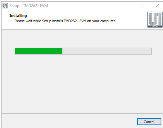
Figure 6: Installation Progress
