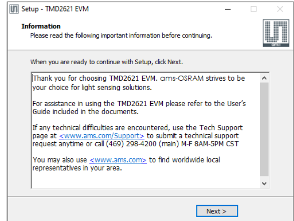
Figure 7: Information Screen
