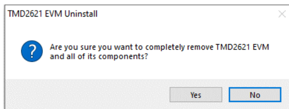
Figure 9: Remove Installation
