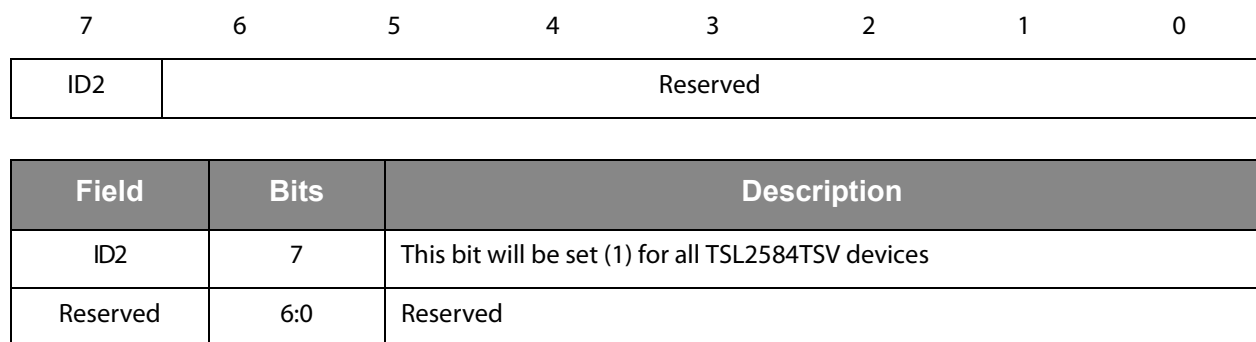
Figure 27: ID2 Register
