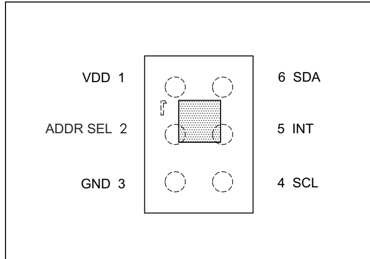
Figure 3: Pin Diagram
