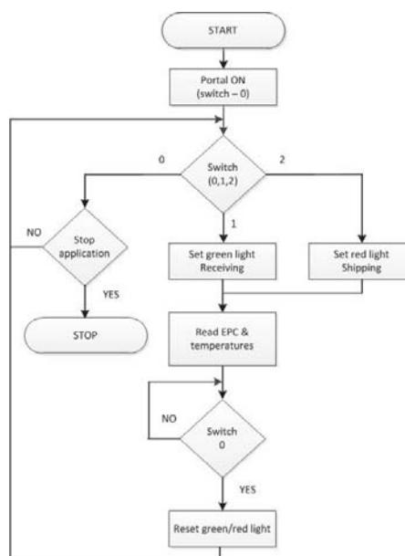
Fig. 3 RFID portal application
