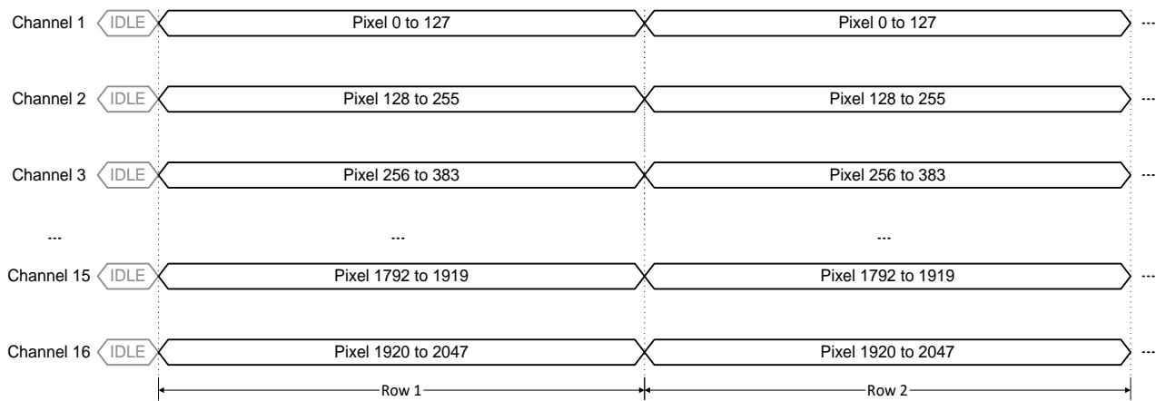
FIGURE 26: PIXEL REMAPPING FOR 16 OUTPUT CHANNELS
