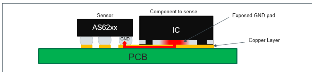
Figure 1 : Copper Connection on Same Layer for Heat Transfer
