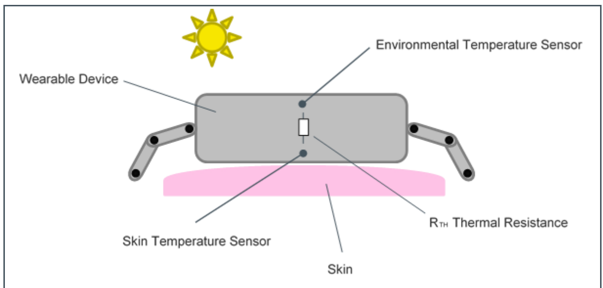
Figure 5: Environmental Sensing
