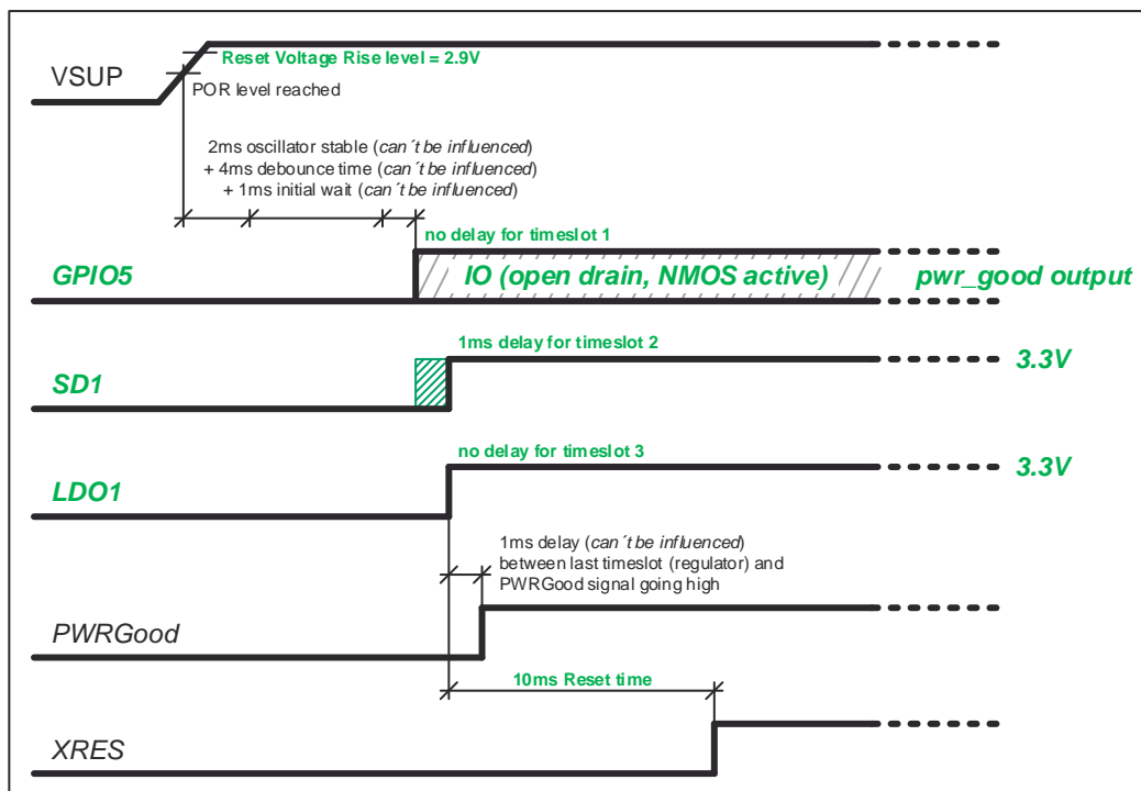
Figure 2: Startup diagram for AS3701B-BWLM-68
