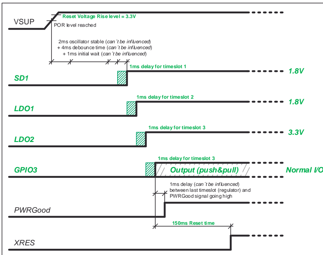
Figure 2: Startup digram for AS3701B-BWLM-05
