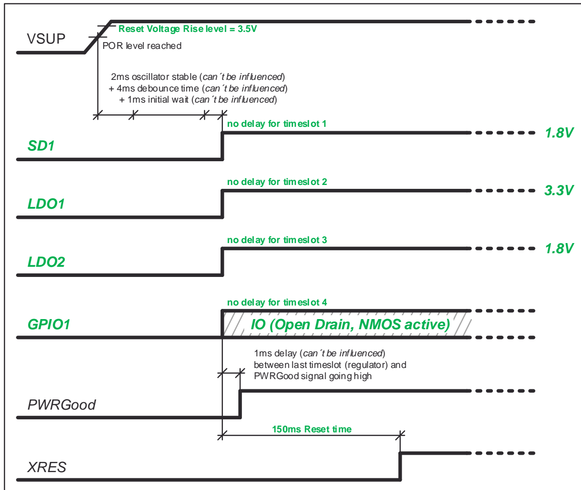
Figure 2: Startup diagram for AS3701B-BWLM-02
