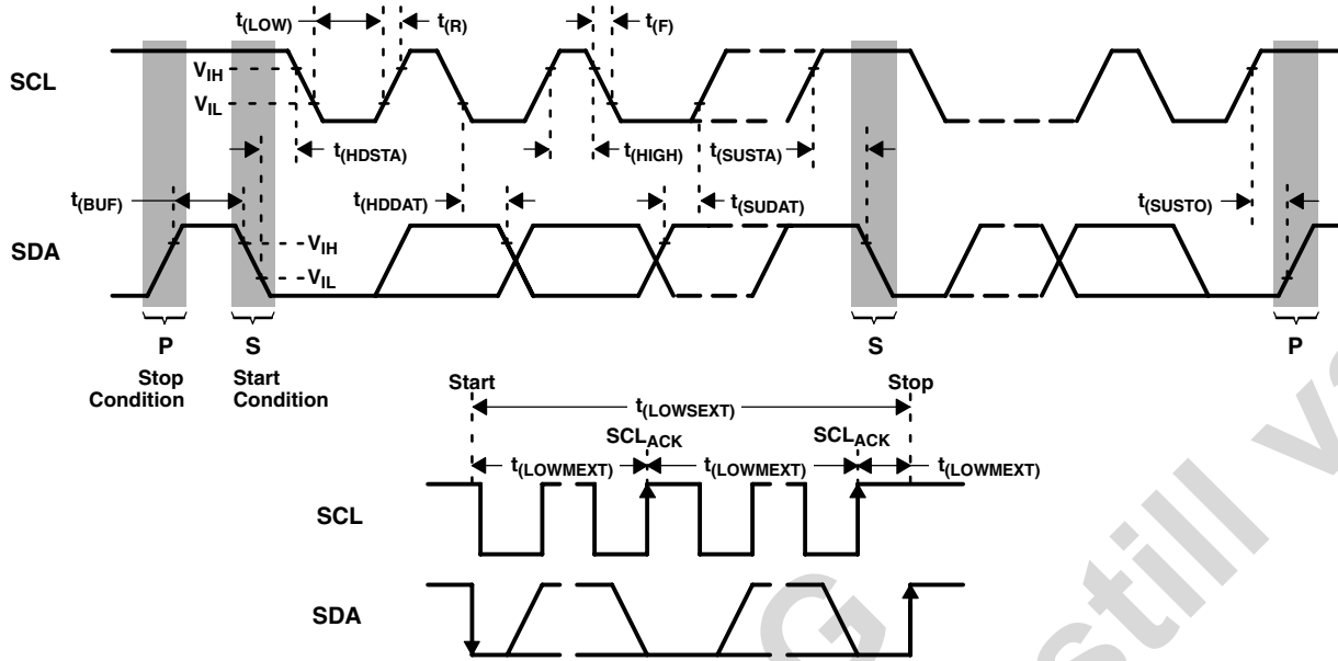
Figure 2. Timing Diagrams
